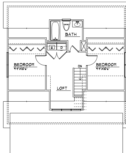
Second Floor 480 Sq. Ft.
