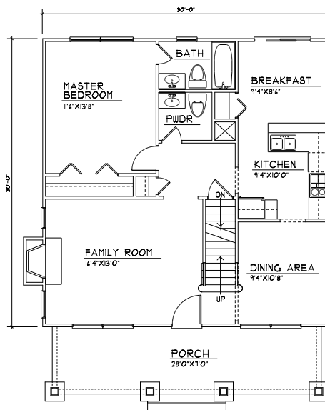
First Floor 900 Sq. Ft. Basement Option
